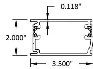
2 MEETING STILE
