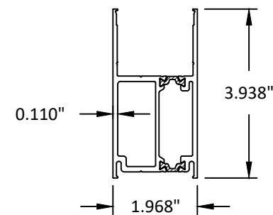
5 TOP RAIL
