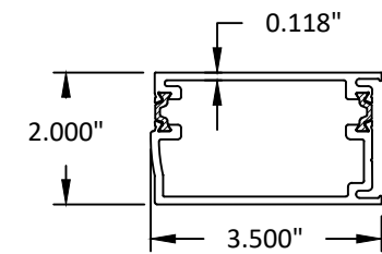
3 MEETING STILE
