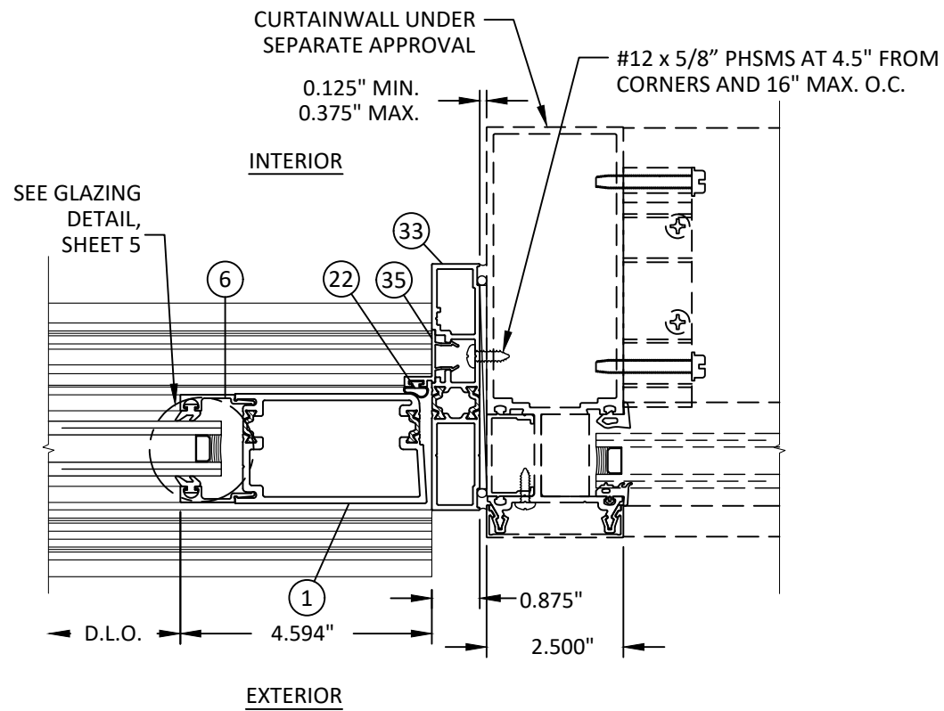
K 7 HORIZONTAL SECTION STANDARD LOCK OR HINGE JAMB THERMAL JAMB SUBFRAME (FLAT) TO CURTAINWALL
