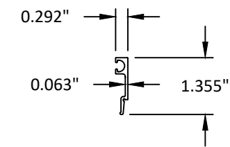
6 GLASS STOP
