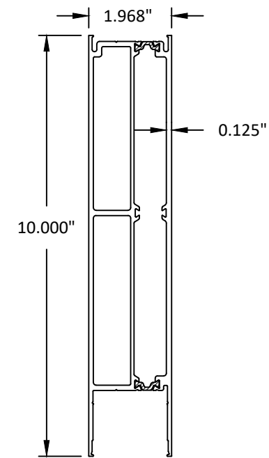
4 10" BOTTOM RAIL
