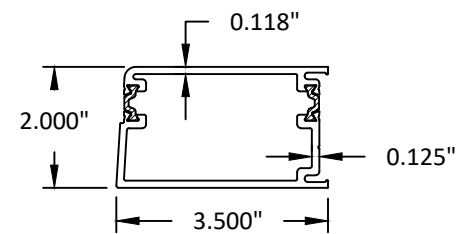
1 VERTICAL STILE
