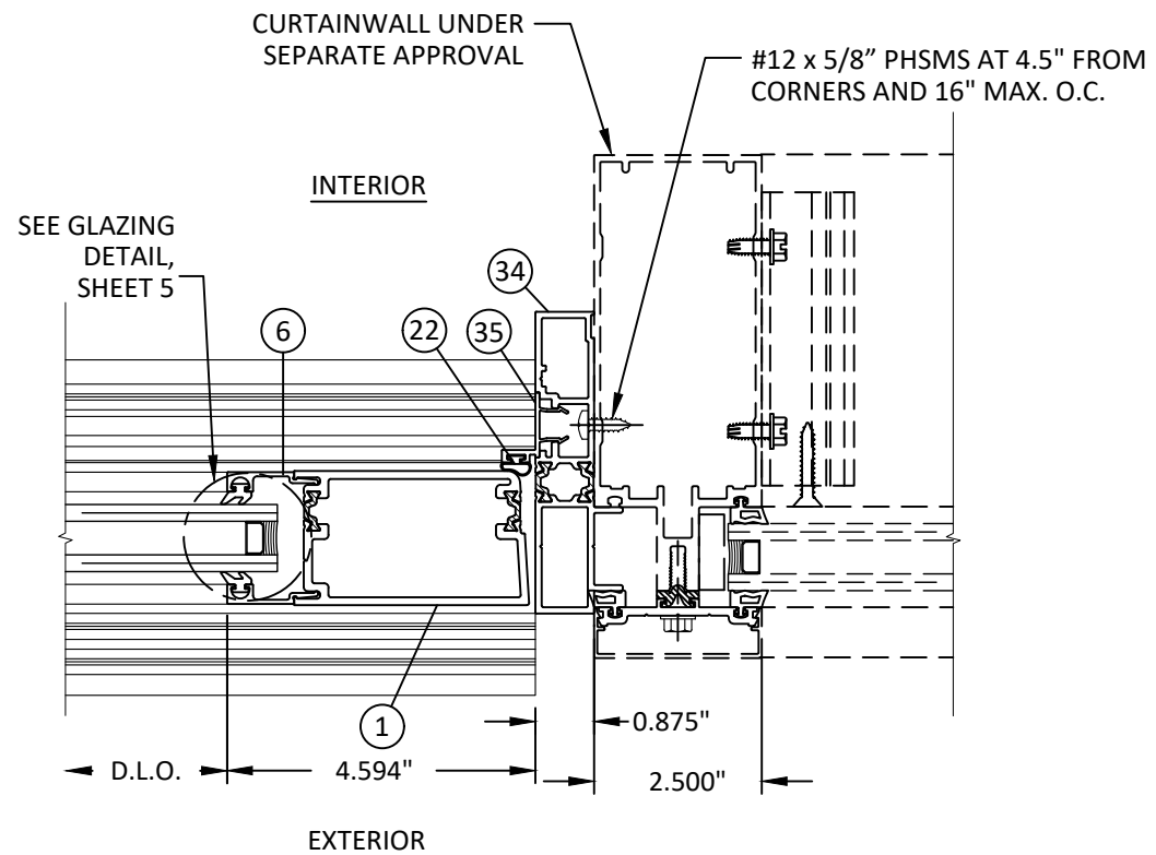
L 7 HORIZONTAL SECTION STANDARD LOCK OR HINGE JAMB THERMAL JAMB SUBFRAME (POCKET) TO CURTAINWALL
